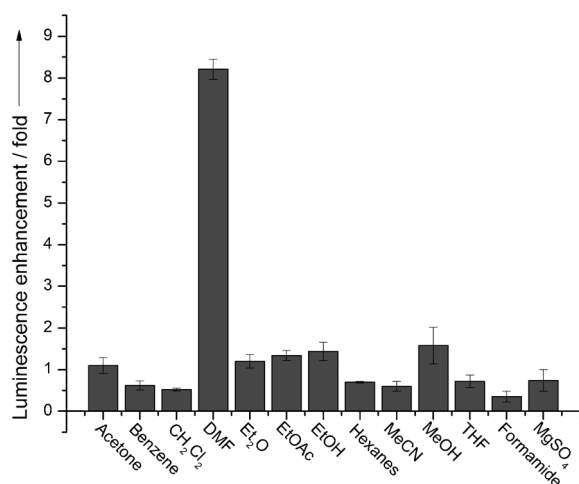
Figure 2. Increase in Eu emission intensity of 2 ( I_{\text{after}}/I_{\text{before}} - 1 ) after incubation for 24 h under various solvent vapors and with anhydrous \text{MgSO}_4 . The intensity is measured at 616 nm. Error bars indicate the standard deviations of three or four parallel experiments.
